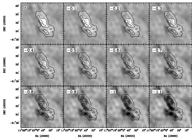
FIG. 5.—Tomographic spectral index images for the bright southeastern rim of the shell G292.2–0.5. The gray scale shows a series of difference images between 1.4 and 2.5 GHz data that have been matched in u - v coverage. For each panel, the trial spectral index is shown at the upper left. Contours in each panel correspond to the 1.4 GHz data, shown in Fig. 2, at levels of 10, 20, and 30 mJy beam -1 . Light (dark) regions of the image indicate that a feature has a more negative (positive) spectral index than the trial value. The transition from light to dark occurs at a spectral index \sim -0.6 .
